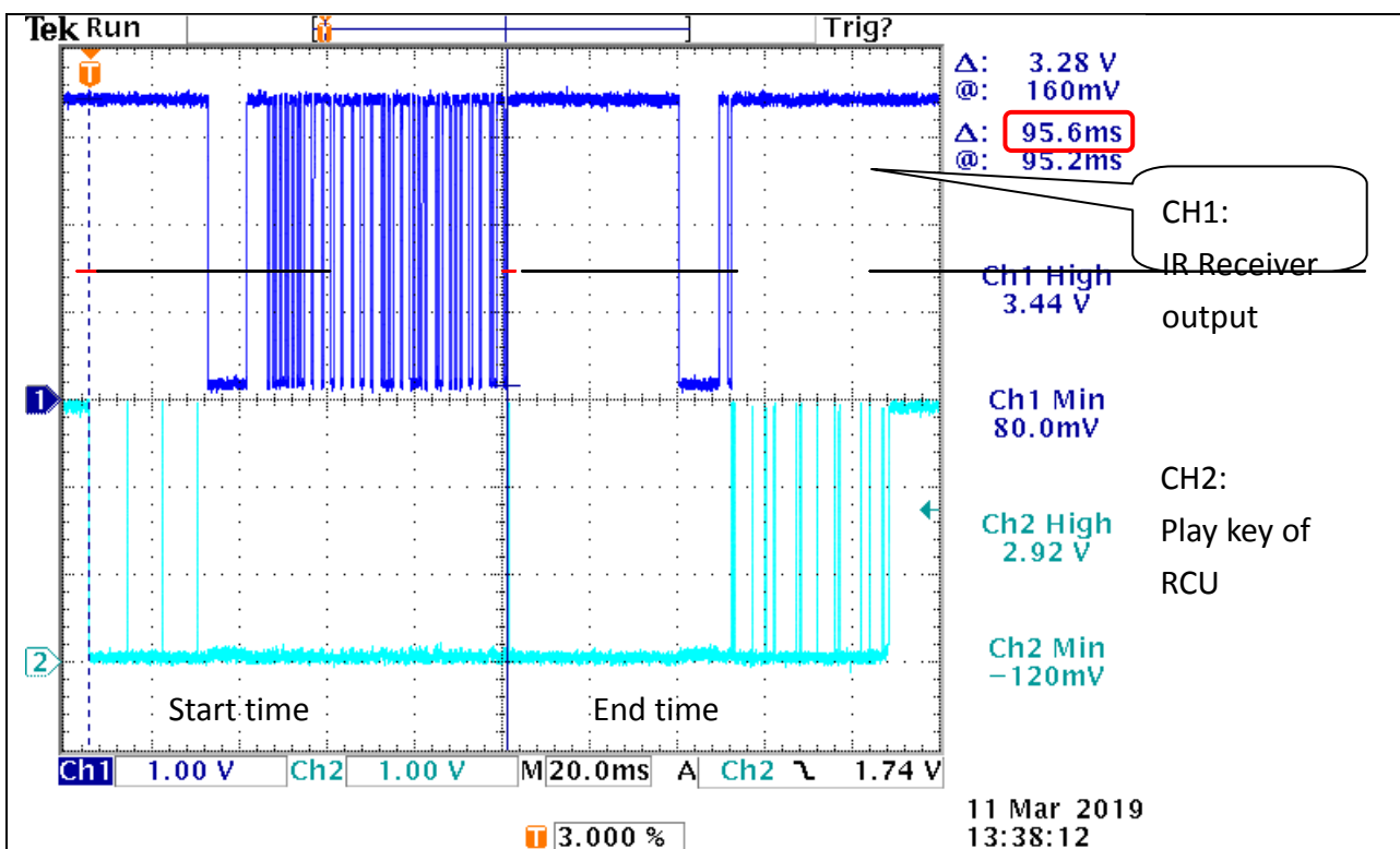
Figure 4: Response time of press play key on the RCU and IR receiver output on the T99X171T00
